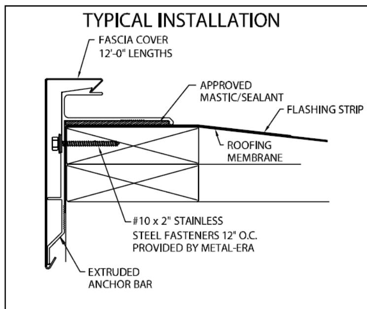
HEAVY GAUGE EXTRUDED FASCIA MB
