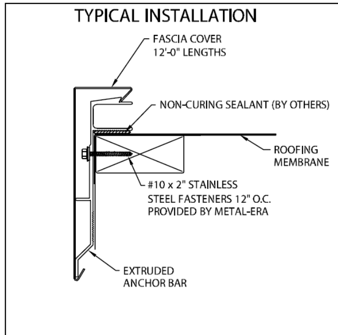
HEAVY GAUGE EXTRUDED FASCIA
