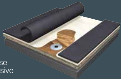
EPDM Fully Adhered with Solvent-Base Adhesive
