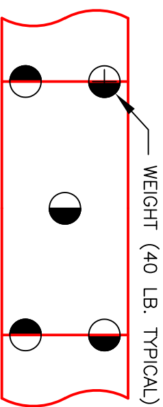
FIGURE 3 INSTALLATION USING 4" O.C. BEADS ON 4' X 8' BOARDS
