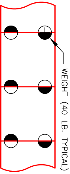
FIGURE 1 INSTALLATION USING 4" O.C. BEADS ON 4' X 4' BOARDS
