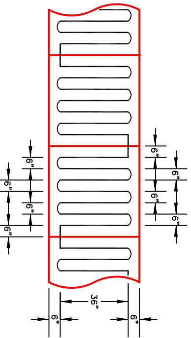
FIGURE 1 INSTALLATION USING 6" O.C. BEADS ON 4' X 4' BOARDS
