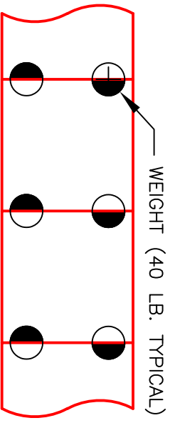
FIGURE 1 INSTALLATION USING 6" O.C. BEADS ON 4' X 4' BOARDS
