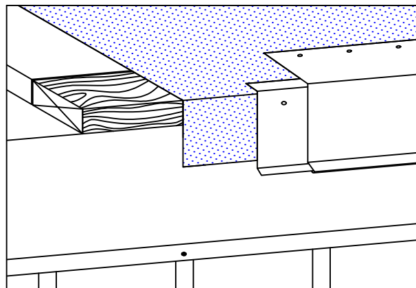
OPTION B - DRIP EDGE OR GRAVEL STOP REFER TO DRIP EDGE DETAILS FOR OPTIONS, AND FOR ADDITIONAL INSTALLATION AND FLASHING REQUIREMENTS
