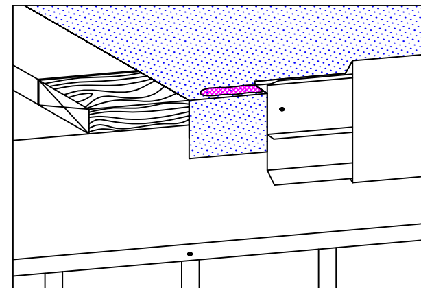
OPTION C - FASCIA EDGE METAL REFER TO DETAIL TP-EM-C116 OR TP-EM-C117 FOR ADDITIONAL INSTALLATION AND FLASHING REQUIREMENTS
