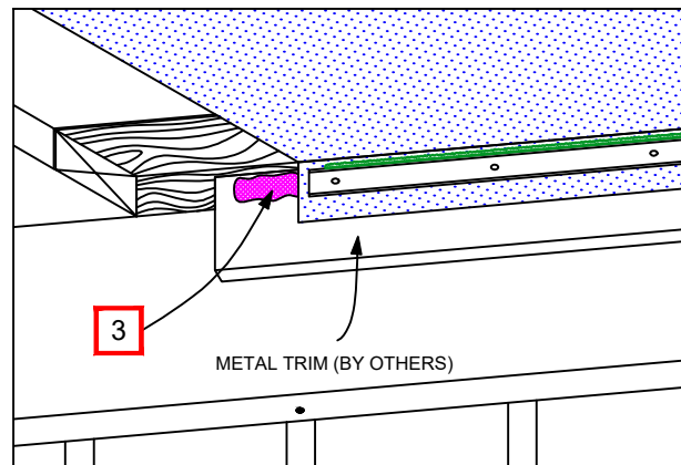
OPTION A - MULEHIDE AP BAR OR ALUMINUM BAR W/ 1-3/4" FASCIA COVER COMBINATION REFER TO DETAIL TP-TM-C610 OR T-TM-C611 FOR ADDITIONAL REQUIREMENTS
