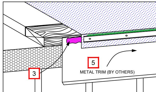
OPTION A - MULEHIDE AP BAR OR ALUMINUM BAR W/ 1-3/4" FASCIA COVER COMBINATION
