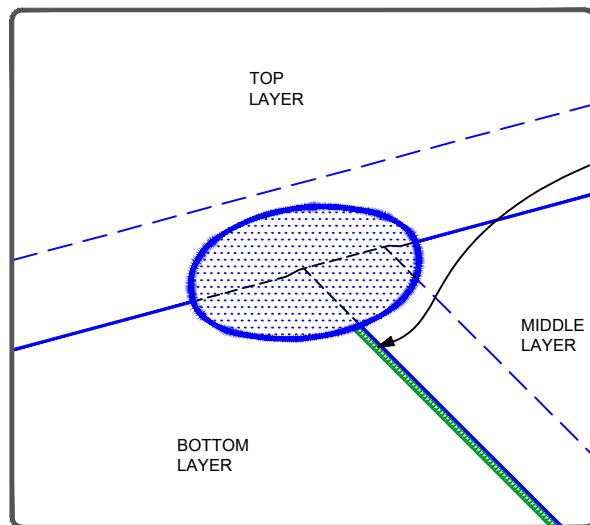
UP SLOPE T-JOINT: ADJOINING SHEET OVERLAPPING END LAP
