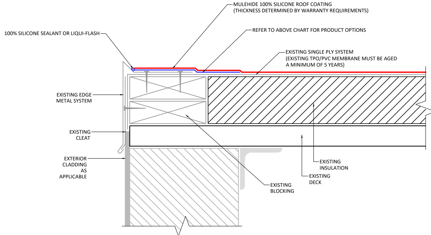
APPLICABLE SYSTEMS (AND MEMBRANES) EXISTING SINGLE PLY ASSEMBLY
