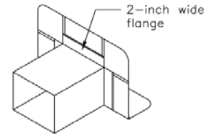
Single Skirt Scupper
