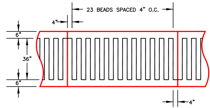
FIGURE 3 INSTALLATION USING 4" O.C. BEADS ON 4' X 8' BOARDS
