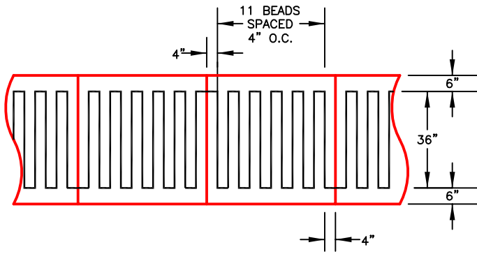
FIGURE 1 INSTALLATION USING 4" O.C. BEADS ON 4' X 4' BOARDS
