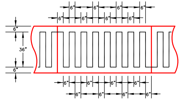
FIGURE 3 INSTALLATION USING 6" O.C. BEADS ON 4' X 8' BOARDS
