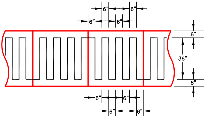
FIGURE 1 INSTALLATION USING 6" O.C. BEADS ON 4' X 4' BOARDS
