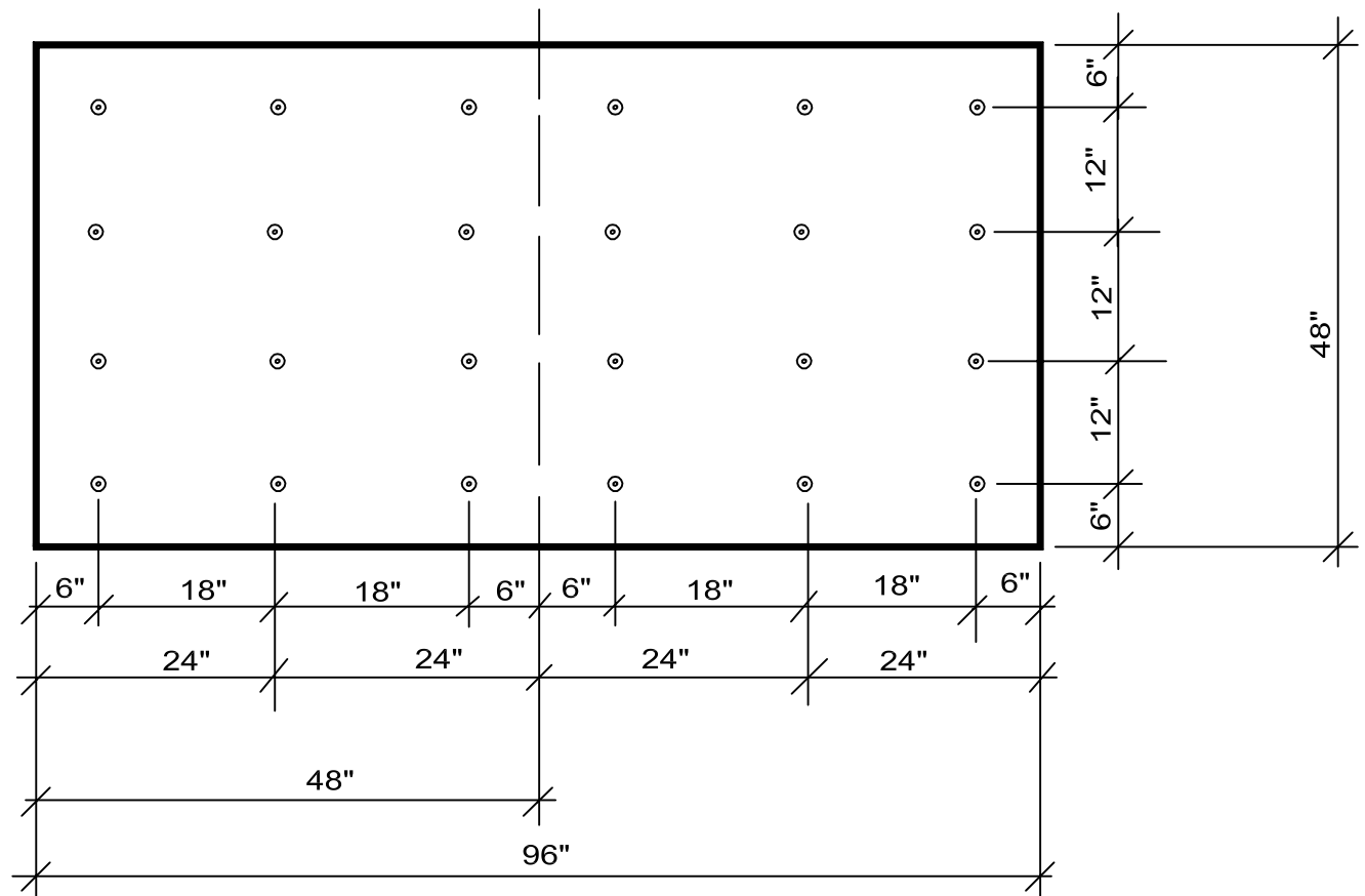
4' X 8' INSULATION ATTACHMENT (1 PER 1.33 SF) STANDARD ATTACHMENT (24 PER BOARD)
