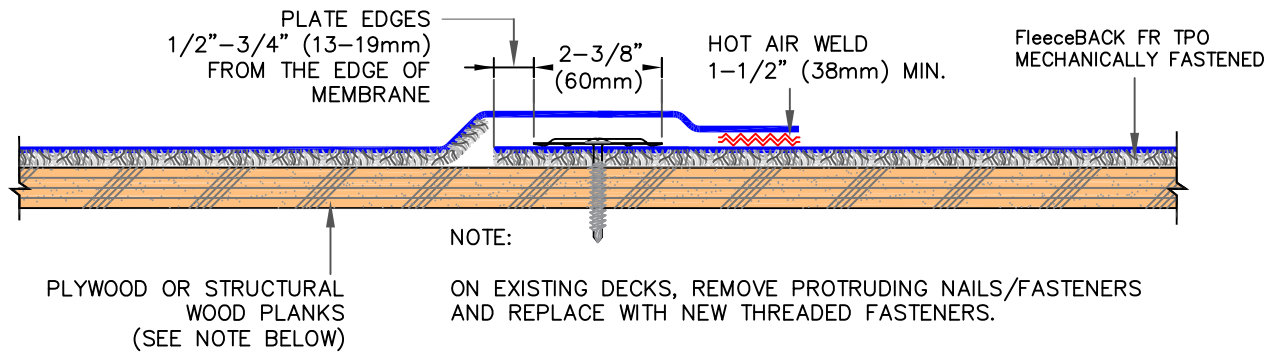
DETAIL A (TYPICAL SEAM)
